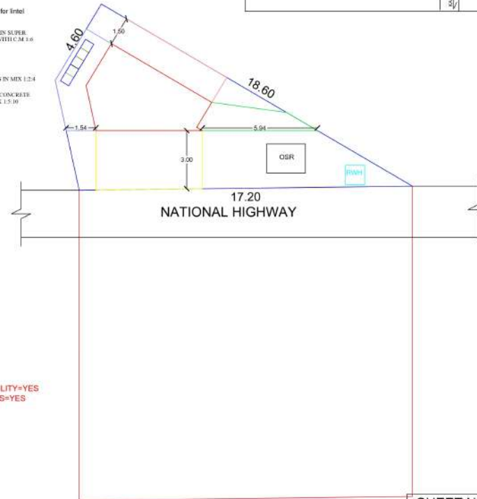
KEY PLAN
