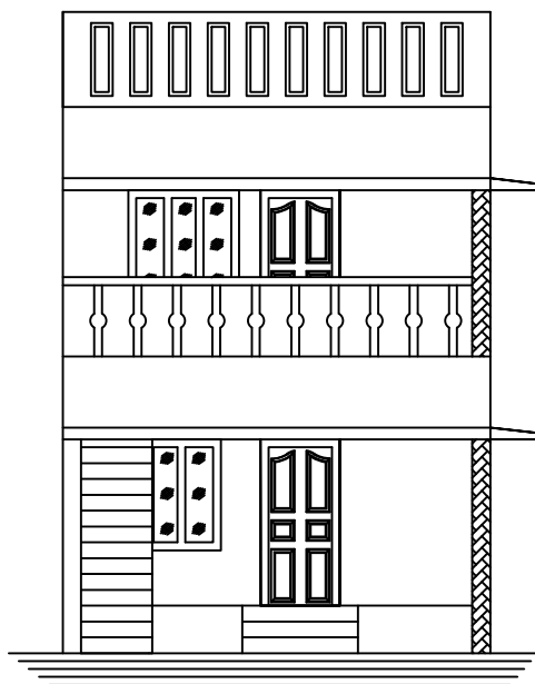
FRONT ELEVATION
