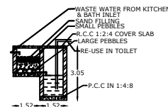
WASTE WATER RECYCLING SYSTEM
