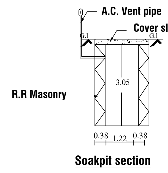
Soakpit section
