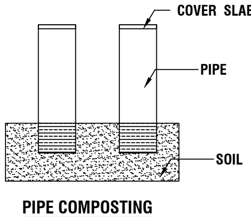
PIPE COMPOSTING
