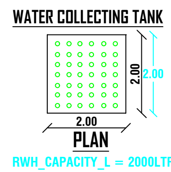
WATER COLLECTING TANK RWHP_CAPACITY_L = 2000LTRS
