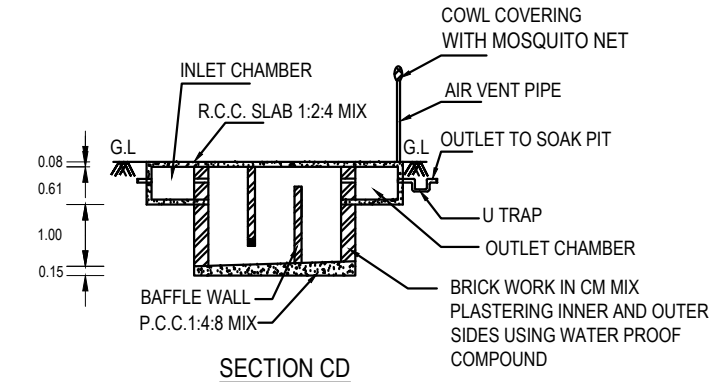
SECTION CD
