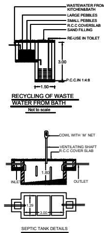
SEPTIC TANK DETAILS
