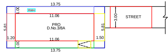
SITE PLAN
