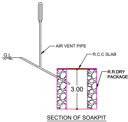
SECTION OF SOAKPIT
