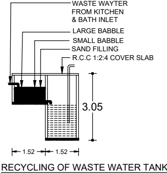
RECYCLING OF WASTE WATER TANK
