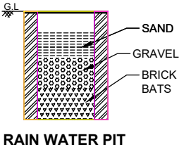
RAIN WATER PIT
