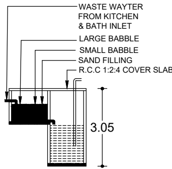
RECYCLING OF WASTE WATER TANK
