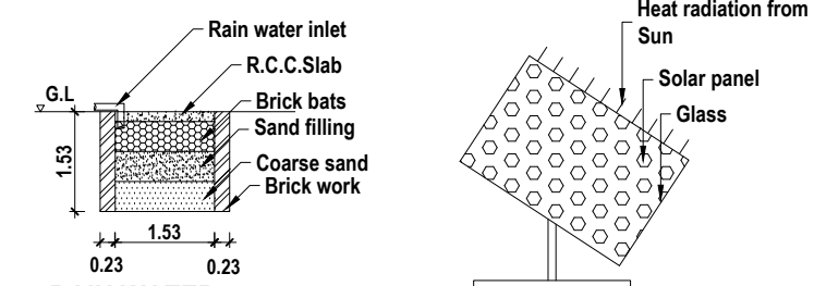
RAIN WATER HARVESTING PIT
