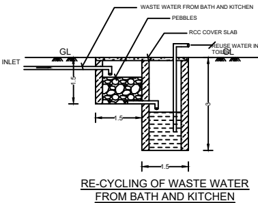
RE-CYCLING OF WASTE WATER FROM BATH AND KITCHEN
