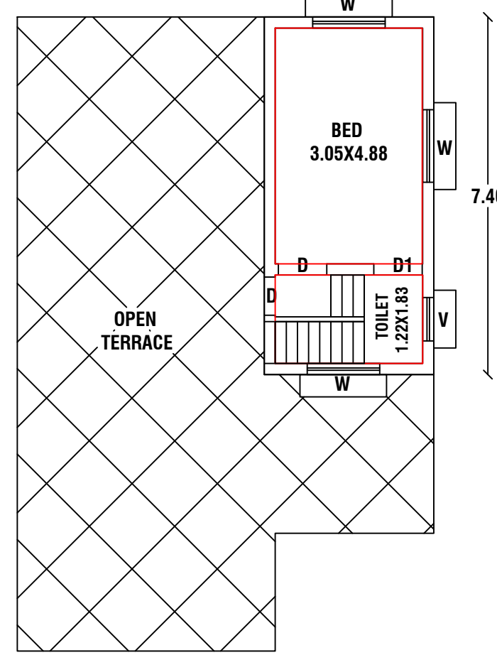
FIRST FLOOR PLAN SCALE 1:100 ALL DIMENSIONS ARE IN METRE
