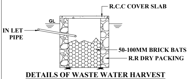
DETAILS OF WASTE WATER HARVEST
