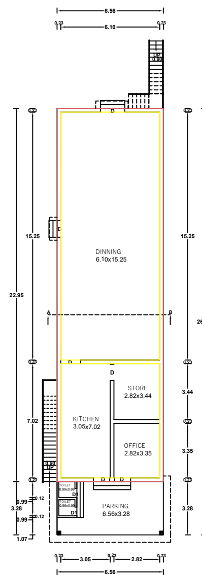
SHOP PLAN
