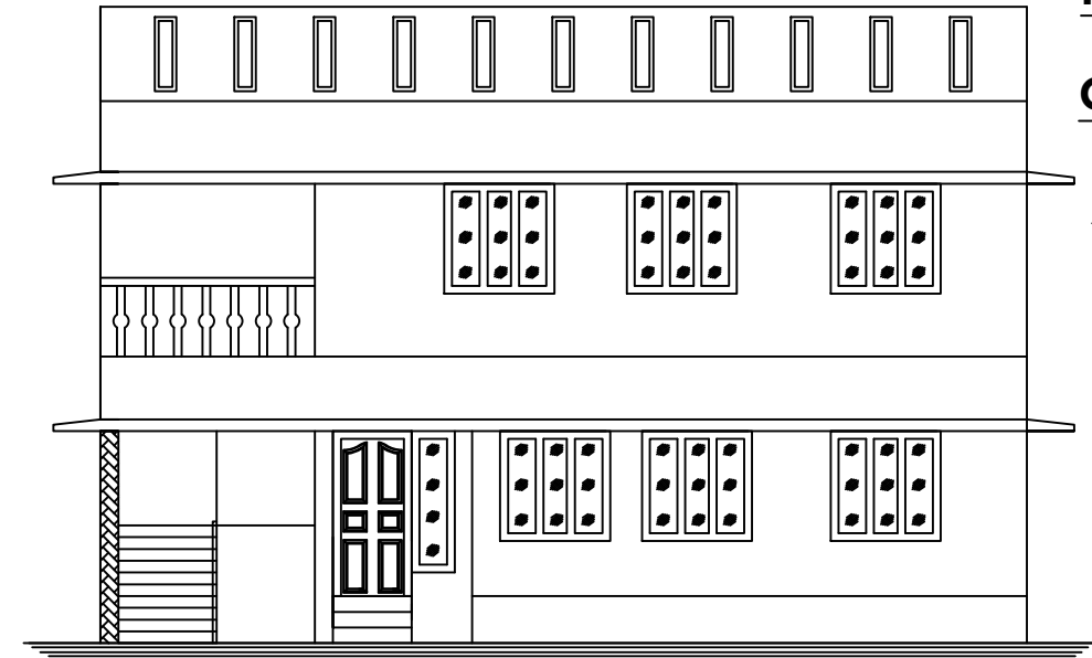
FRONT ELEVATION
