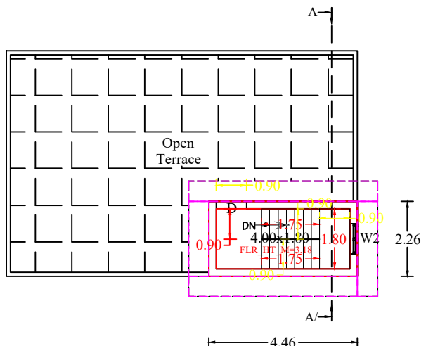
HEAD ROOM PLAN
