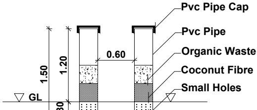
PIPE COMPOST PIT
