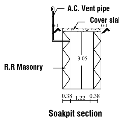
Soakpit section
