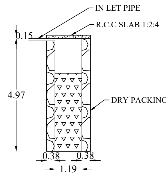
WASTE WATER TANK
