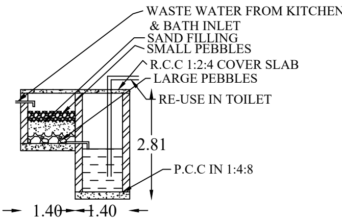
RECYCLING OF WASTE WATER KITCHEN & BATHROOM
