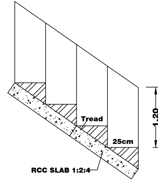
STAIR DETAILS
