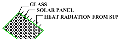
SOLAR SYSTEM
