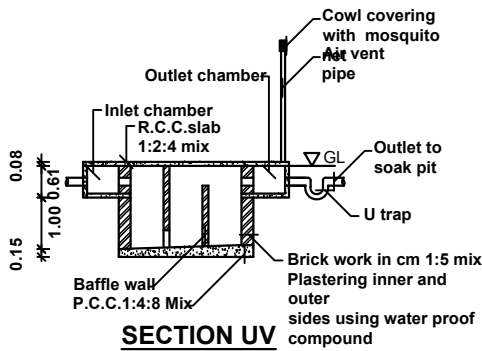
SECTION UV
