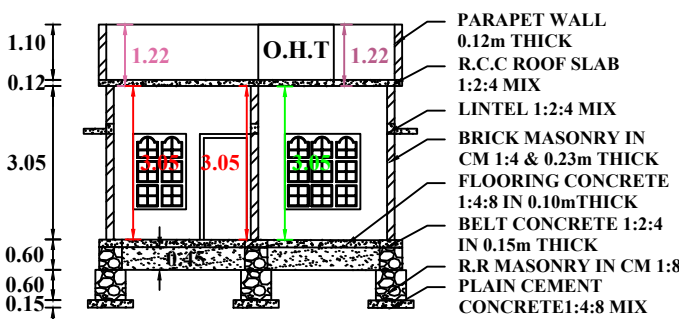
SECTION ON X-Y
