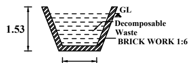
WASTE PIT
