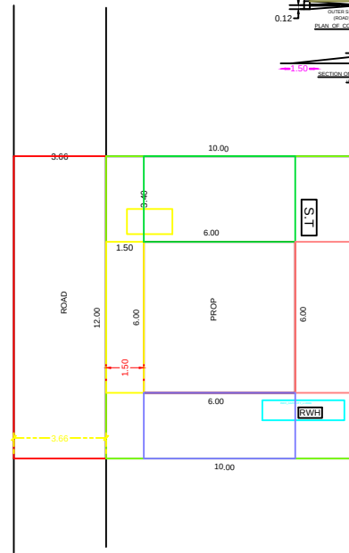
SITE PLAN
