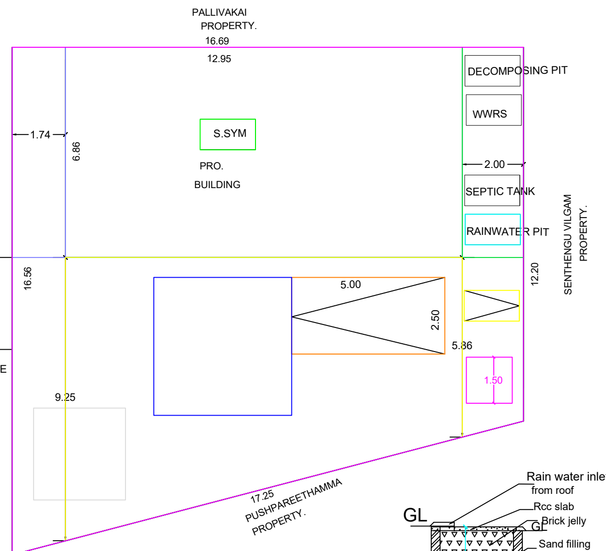
RAIN WATER HARVESTING PIT
