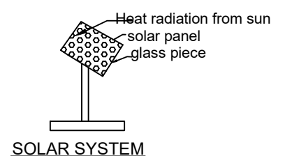
SOLAR SYSTEM
