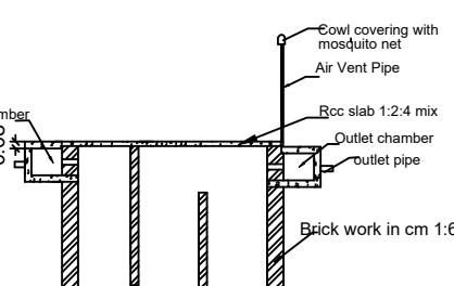
SECTION ON XY
