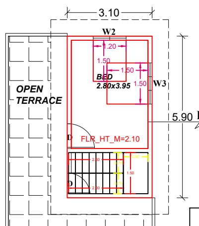
F.F.PLAN (ASBESTOS ROOF)
