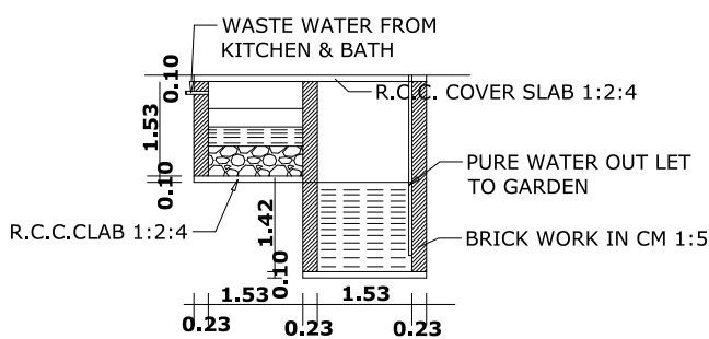
RECYCLING OF WASTE WATER SYSTEM
