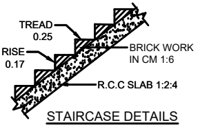
STAIRCASE DETAILS
