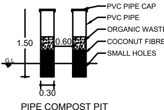
PIPE COMPOST PIT
