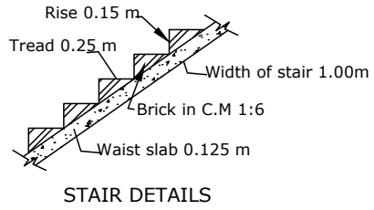
STAIR DETAILS
