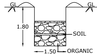
COMPOST PIT
