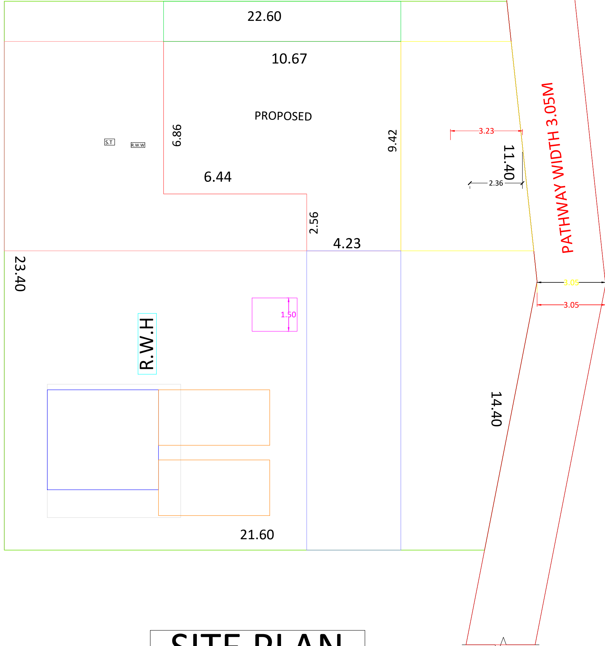
SITE PLAN
