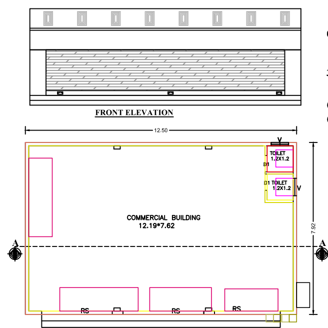
BLOCK -1 GROUND FLOOR PLAN
