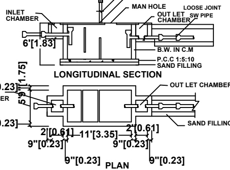
SEPTIC TANK:
