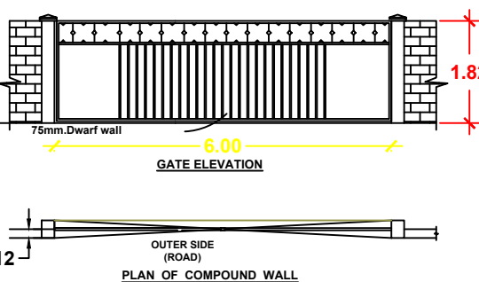
PLAN OF COMPOUND WALL
