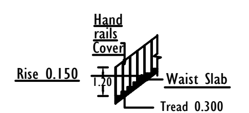
STAIRCASE DETAILS
