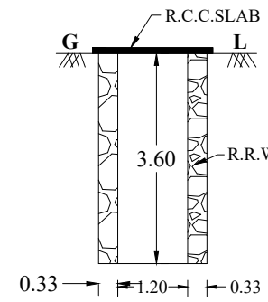
LEACHPIT
