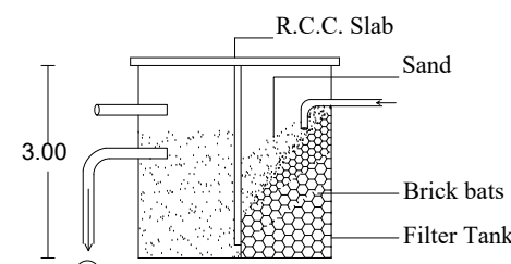
RAINWATER HARVESTING
