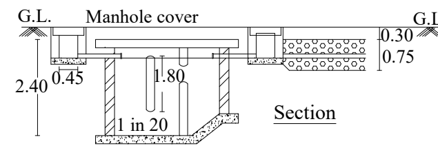
LEACHPIT
