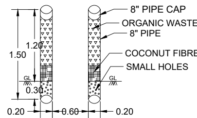
PIPE COMPOSITE PIT NOT TO SCALE
