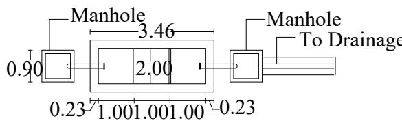
Details Of Septic Tank
