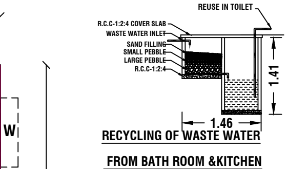
RECYCLING OF WASTE WATER
