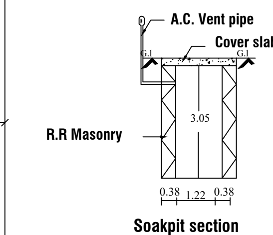
Soakpit section
