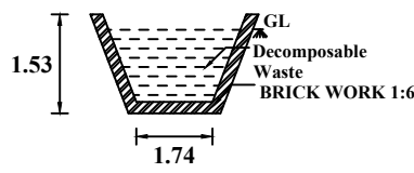
WASTE PIT
