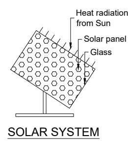
SOLAR SYSTEM
