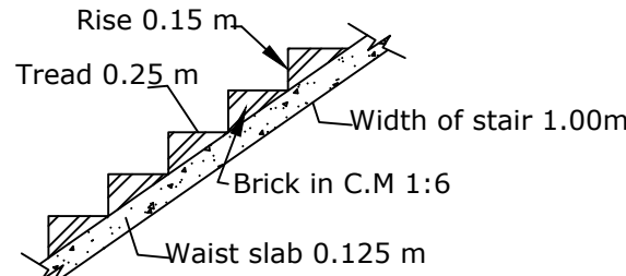
STAIR DETAILS
