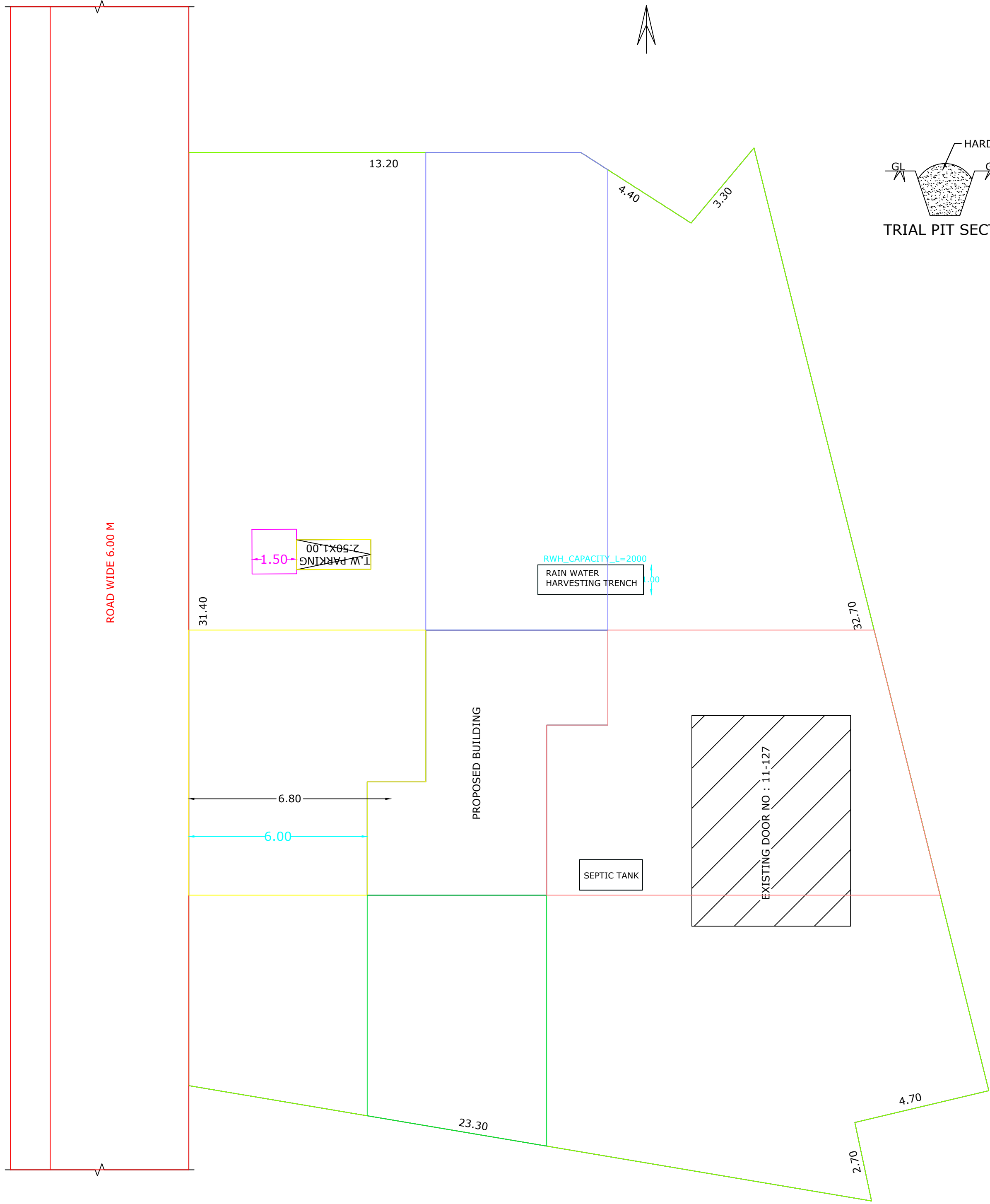
SITE PLAN
