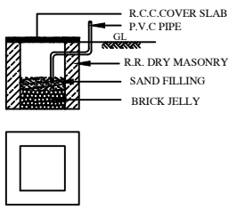
RAIN WATER HARVEST ARRANGEMENTS
