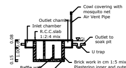
SECTION UV
