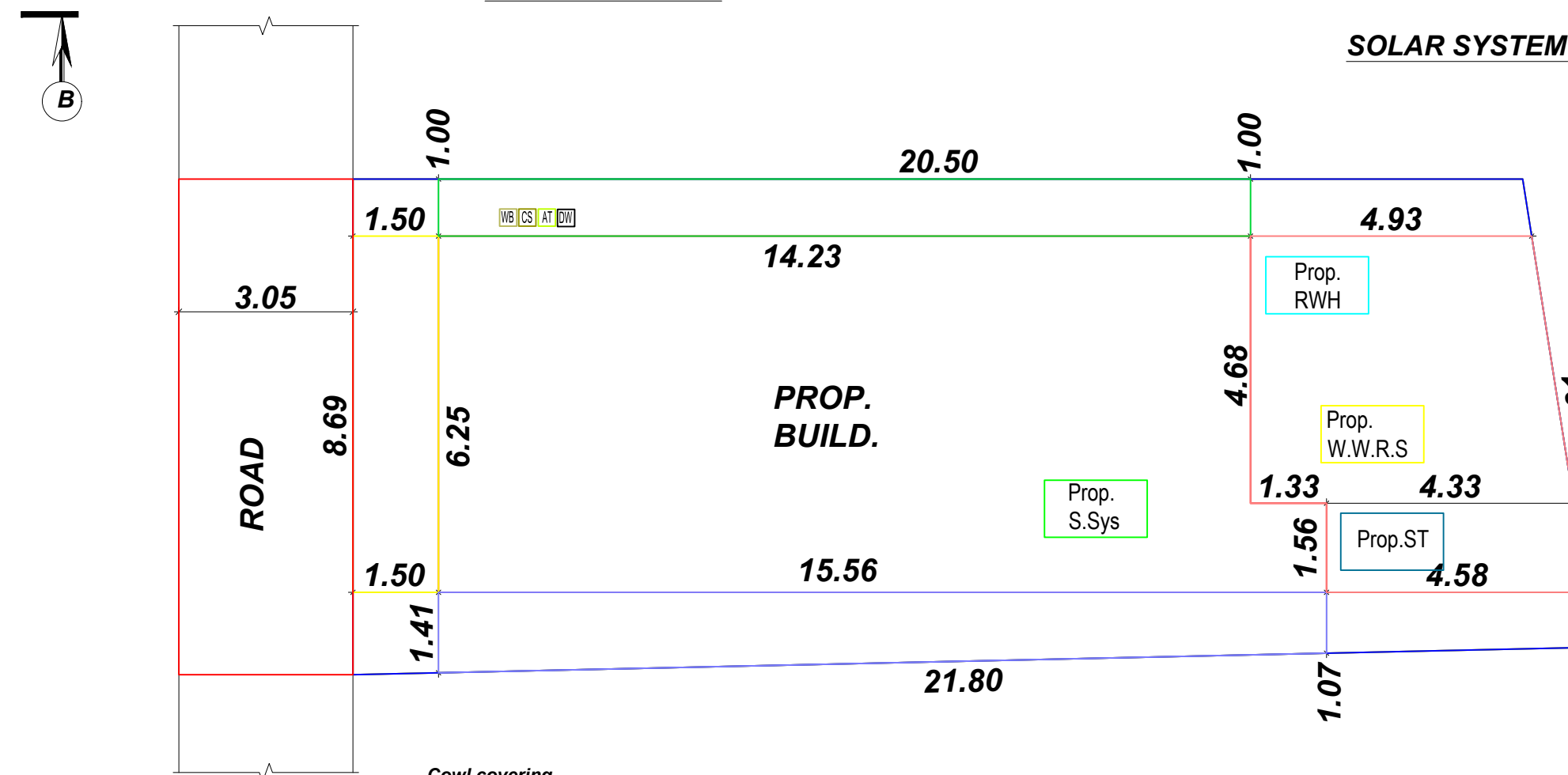
SITE PLAN
