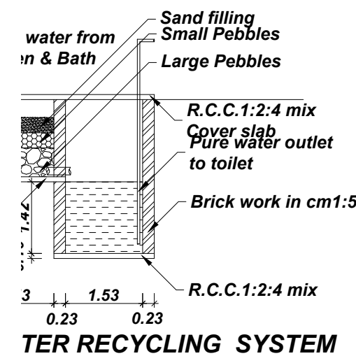
WATER RECYCLING SYSTEM
