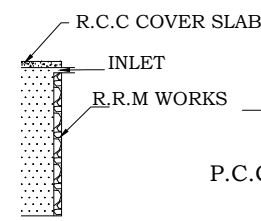
WATER TANK
