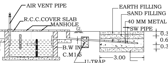
SECTION OF DISPERSION TRENCH
