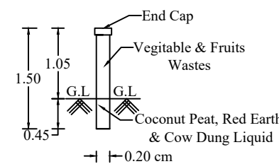
PIPE COMPOSTER
