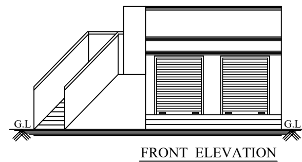
FRONT ELEVATION
