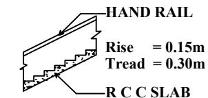
DETAILS OF STAIR CASE
