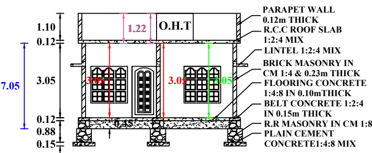
SECTION ON X-Y
