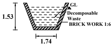
WASTE PIT
