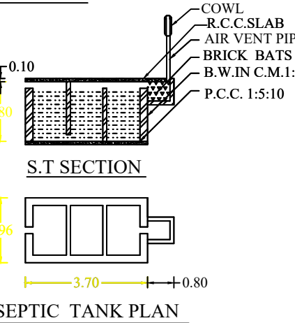
SEPTIC TANK PLAN
