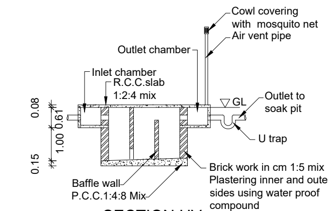
SECTION UV
