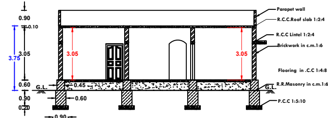
SECTION ON A-B
