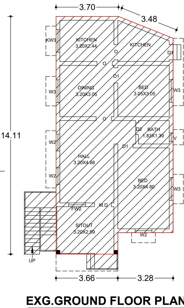
EXG.GROUND FLOOR PLAN
