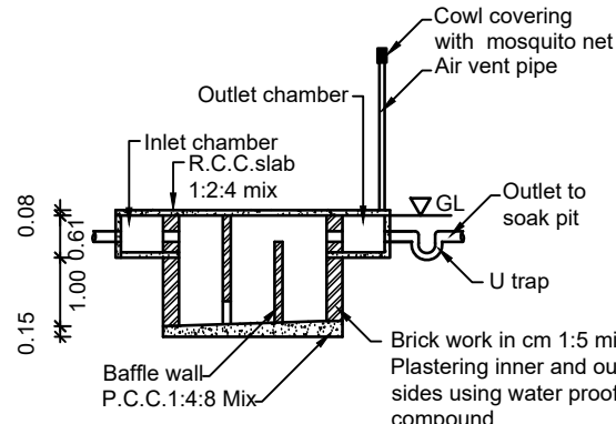
SECTION UV
