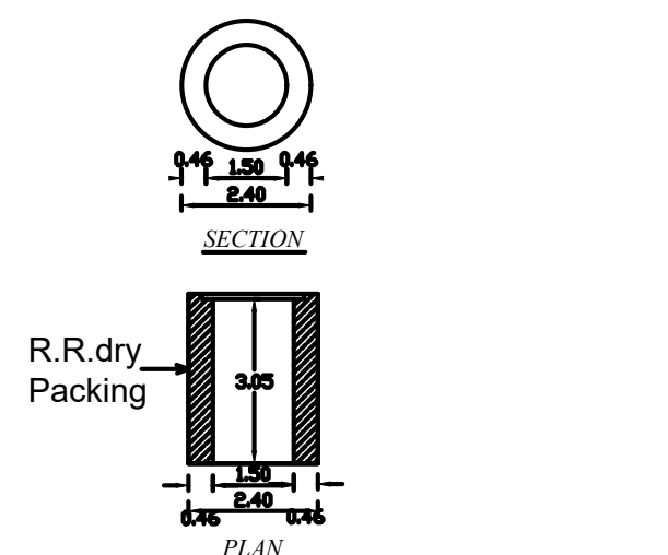
RAIN WATER HARVESTING ARRANGEMENT
