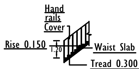
STAIRCASE DETAILS
