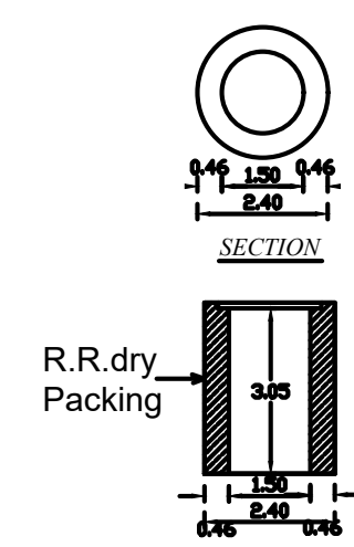
RAIN WATER HARVESTING ARRANGEMENT NOT TO SCALE
